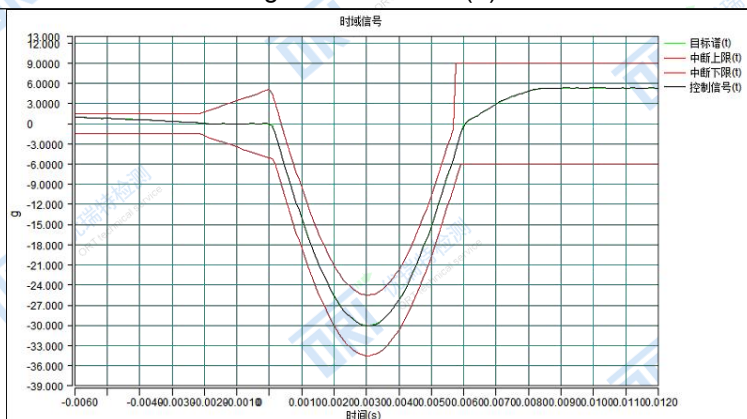
Fig.92 Test Curve (-)
