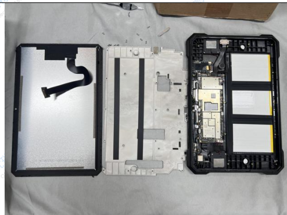
Fig.8 Appearance inspection after test
