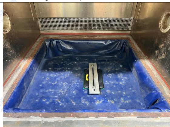
Fig.88 Test setup (X axis)
