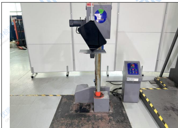
Fig.64 Test setup- Corner (5)
