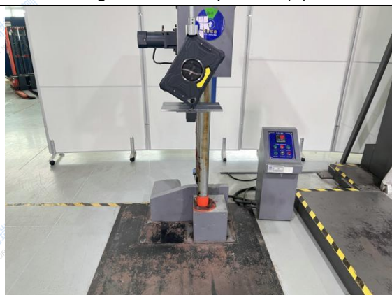
Fig.60 Test setup- Corner (1)
