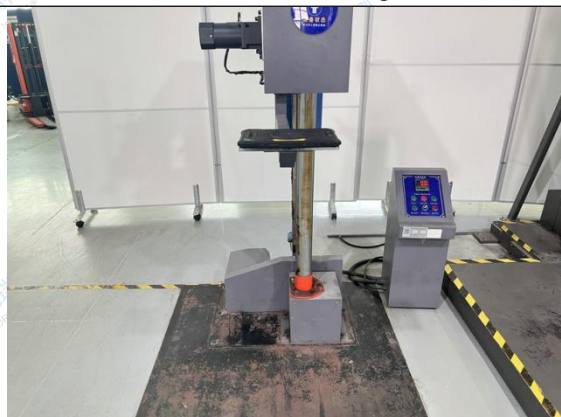
Fig.54 Test setup- Face (1)
