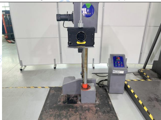
Fig.58 Test setup- Face (5)
