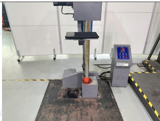
Fig.55 Test setup- Face (2)
