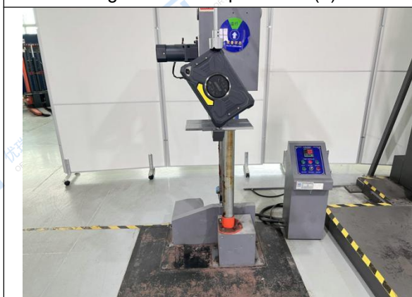
Fig.66 Test setup- Corner (7)
